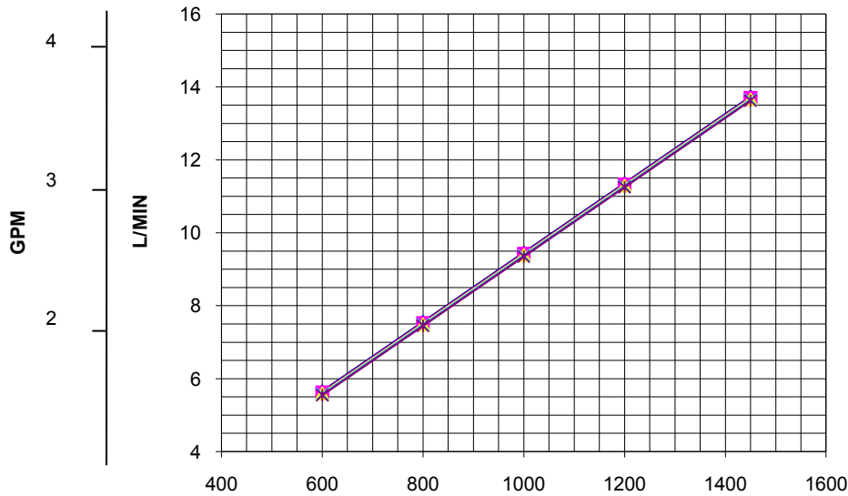
CAUDAL UTIL - USEFUL FLOW RATE
