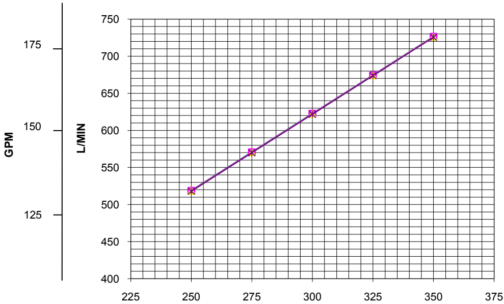
CAUDAL UTIL - USEFUL FLOW RATE
